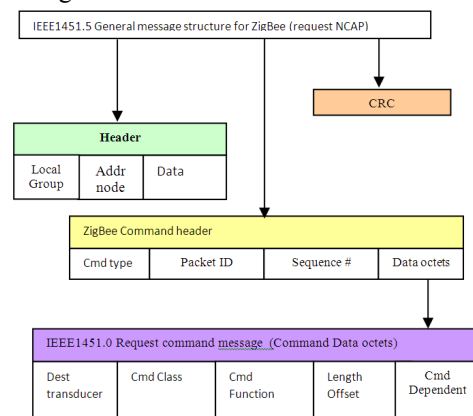
Fig1. IEEE1451 request message structure
